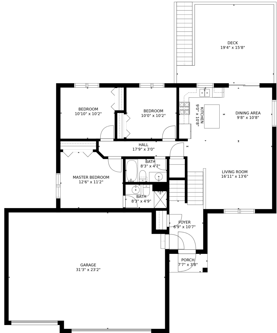
FLOOR 2
